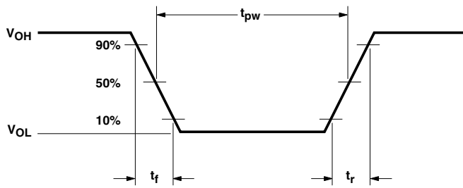
Figure 7. RXD output waveform.
