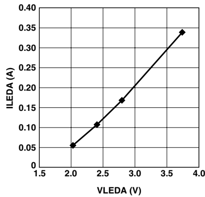
Figure 3. Typical 875 nm LED VLED vs. ILED at room temperature.
