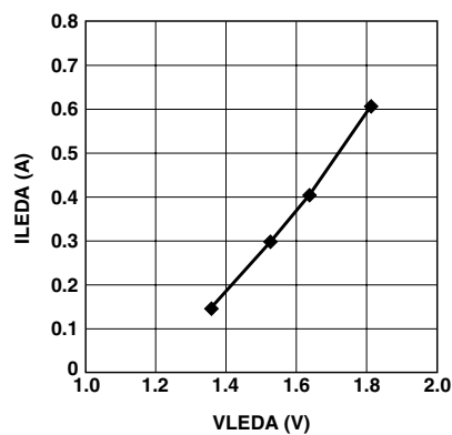
Figure 5. Typical 940 nm LED VLED vs. ILED at room temperature performance.
