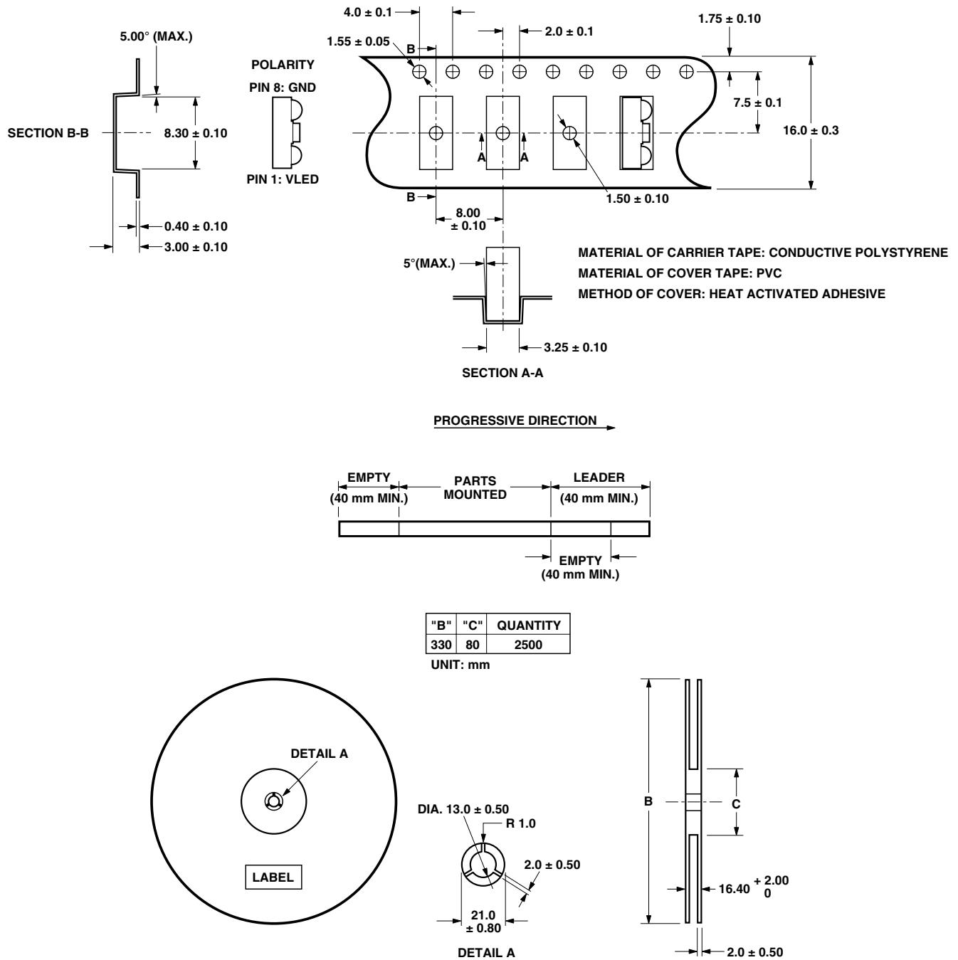
Figure 13. Tape and reel dimensions.
