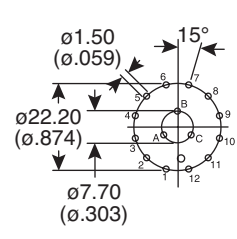
3 Pole Printed Circuit Layout
