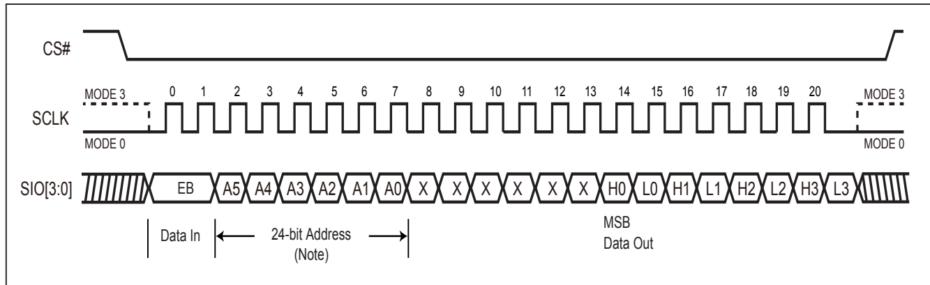
Figure 5. Fast QPI Read Mode (FASTRDQ) (Command EBH)
