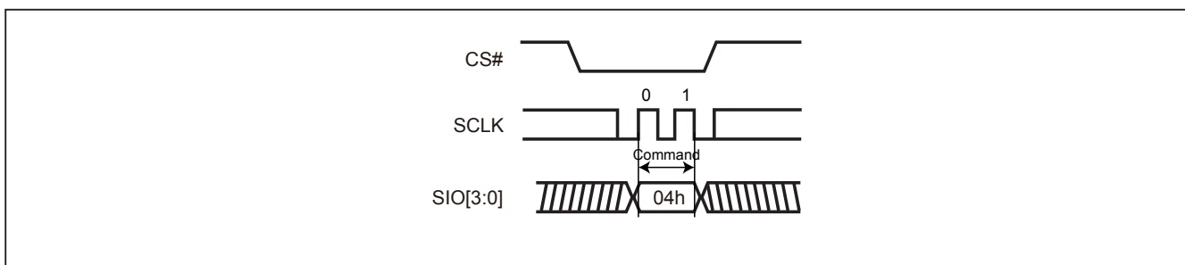
Figure 9. Write Disable (WRDI) Sequence (Command 04) (QPI Mode)
