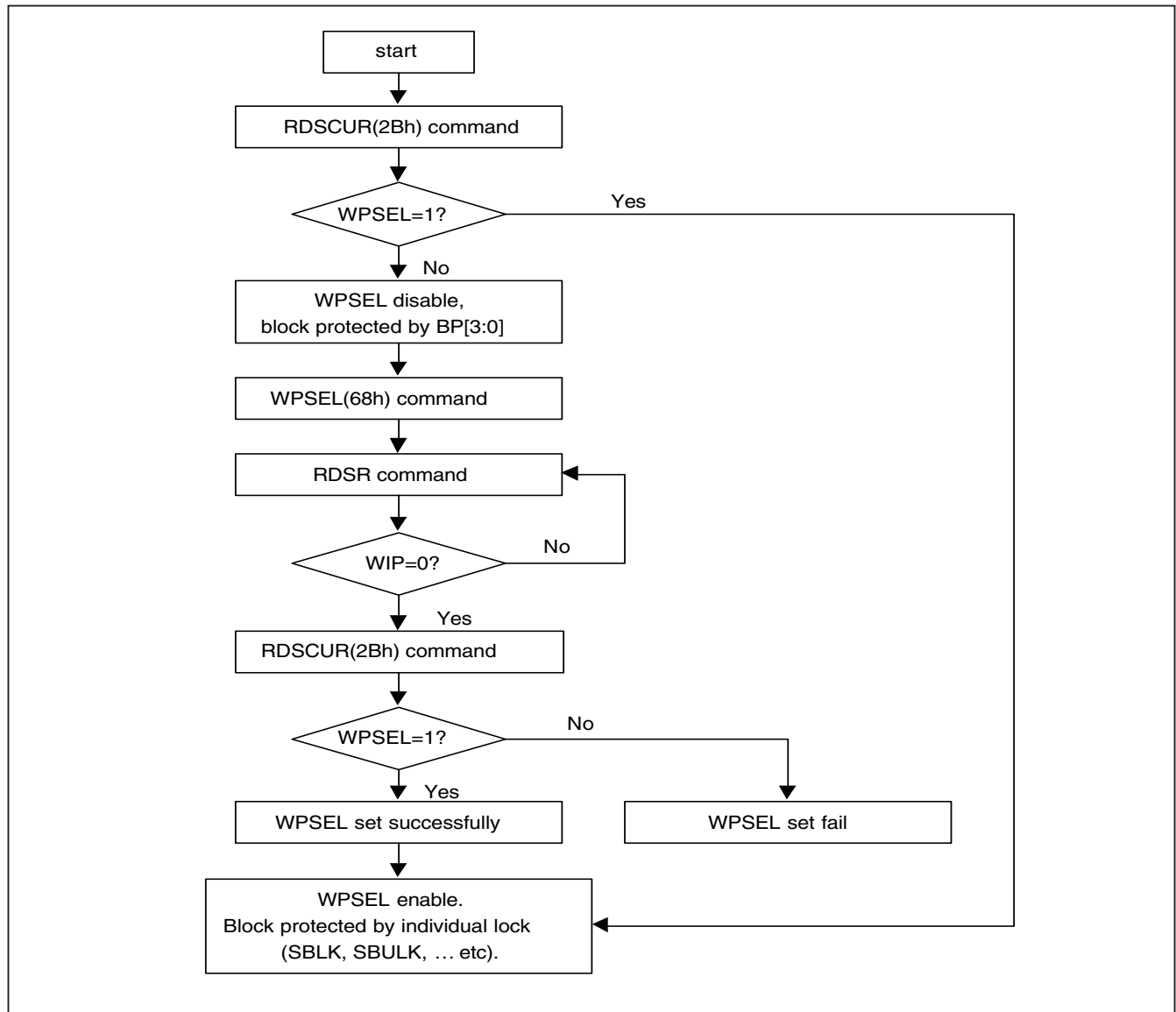
Figure 49. WPSEL Flow
