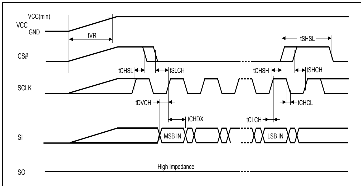
Figure 43. AC Timing at Device Power-Up
