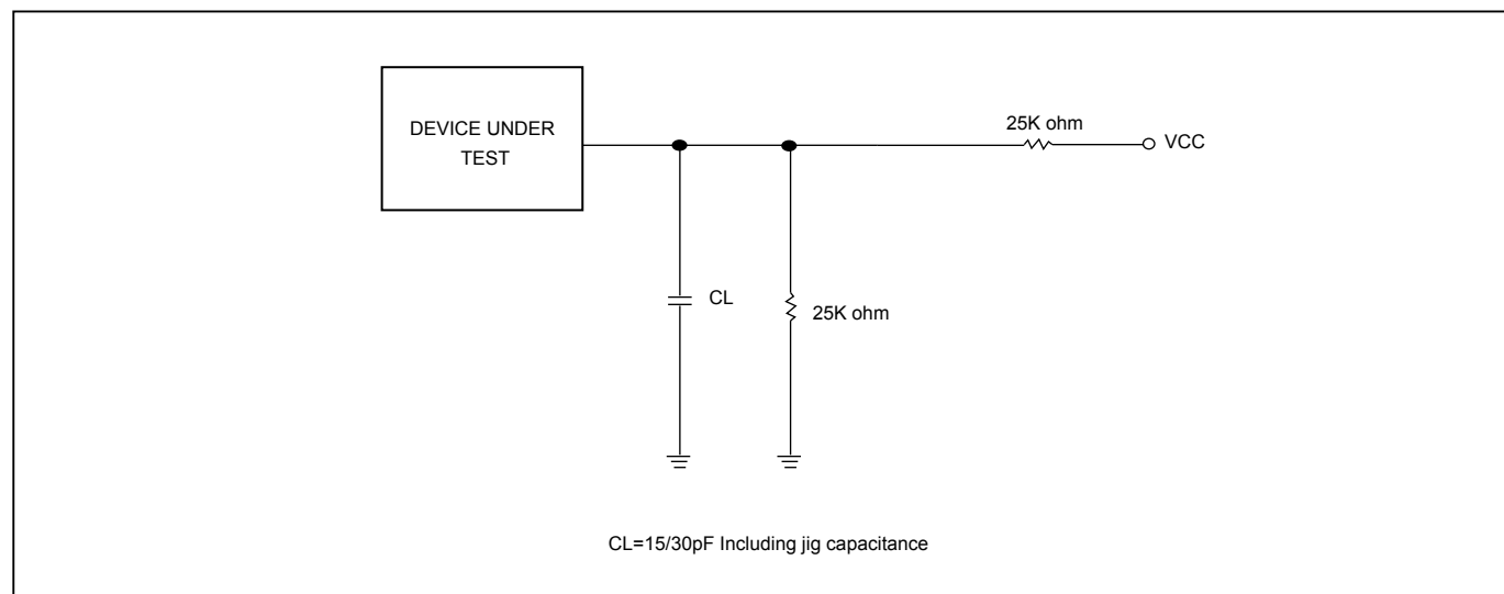
Figure 42. Output Loading
