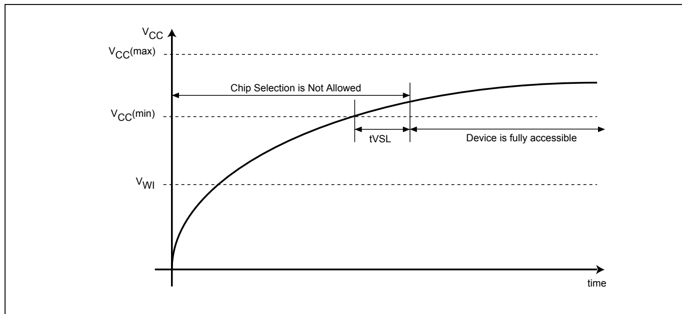
Figure 45. Power-up Timing
