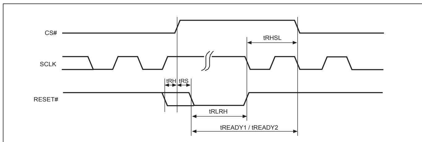
Figure 71. RESET Timing
