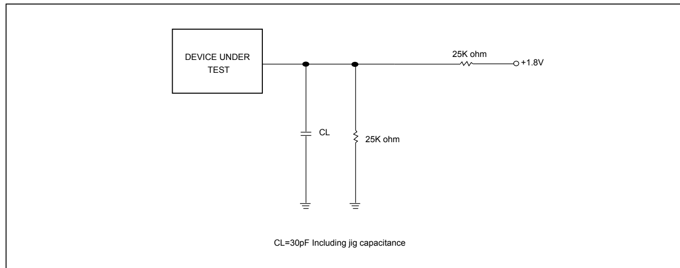
Figure 107. OUTPUT LOADING
