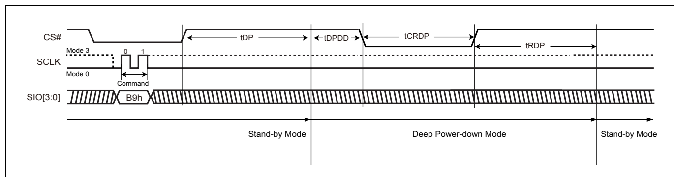
Figure 54. Deep Power-down (DP) Sequence and Release from Deep Power-down Sequence (QPI Mode)
