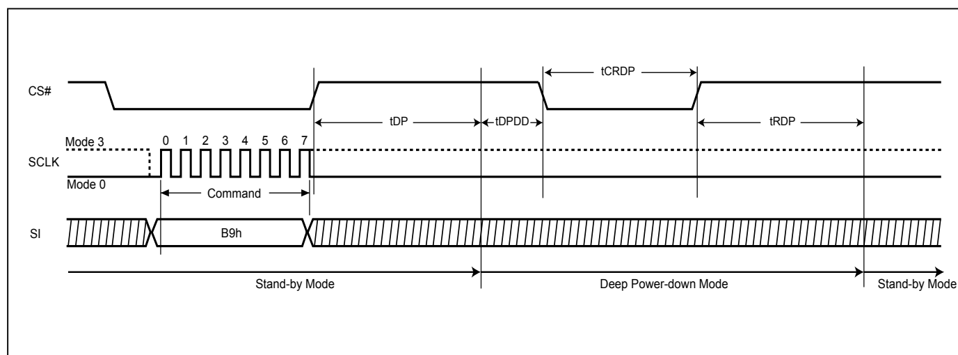
Figure 55. Deep Power-down (DP) Sequence and Release from Deep Power-down Sequence (SPI Mode)
