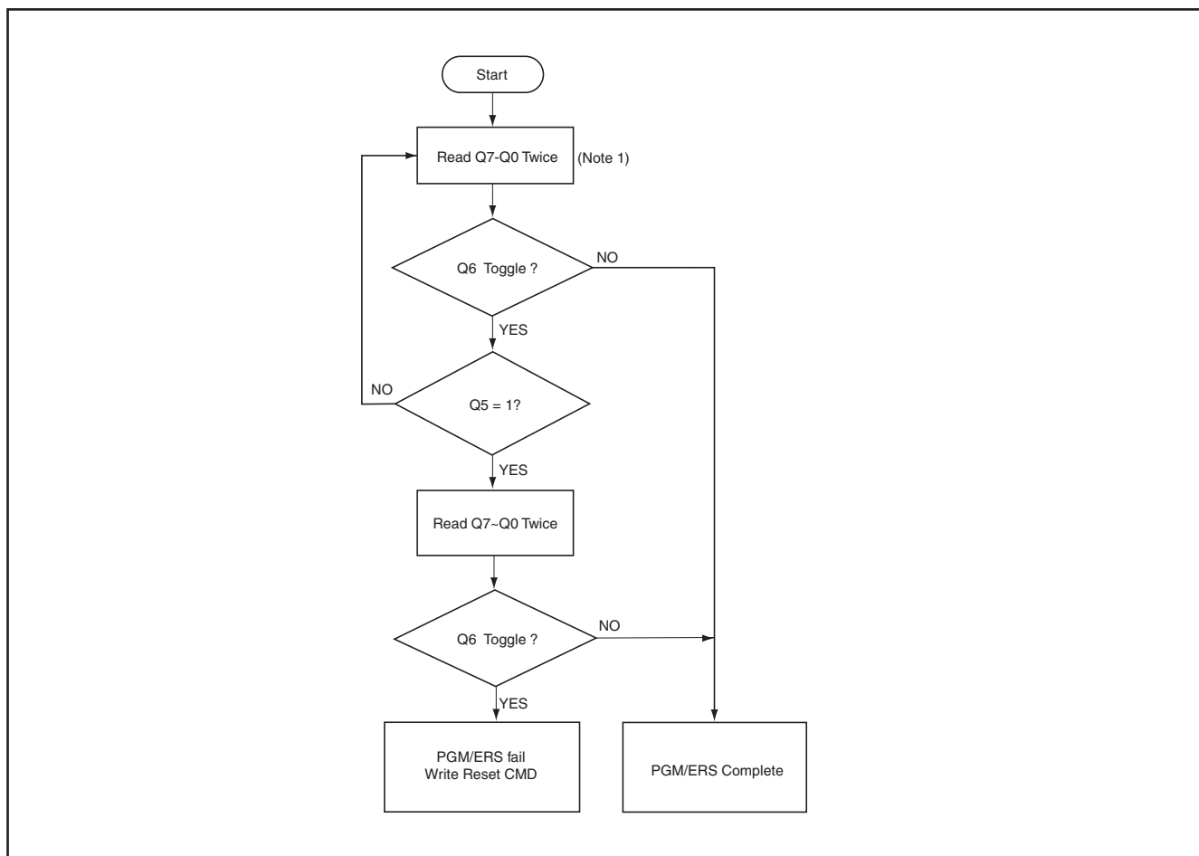
Figure 17. TOGGLE BIT ALGORITHM
