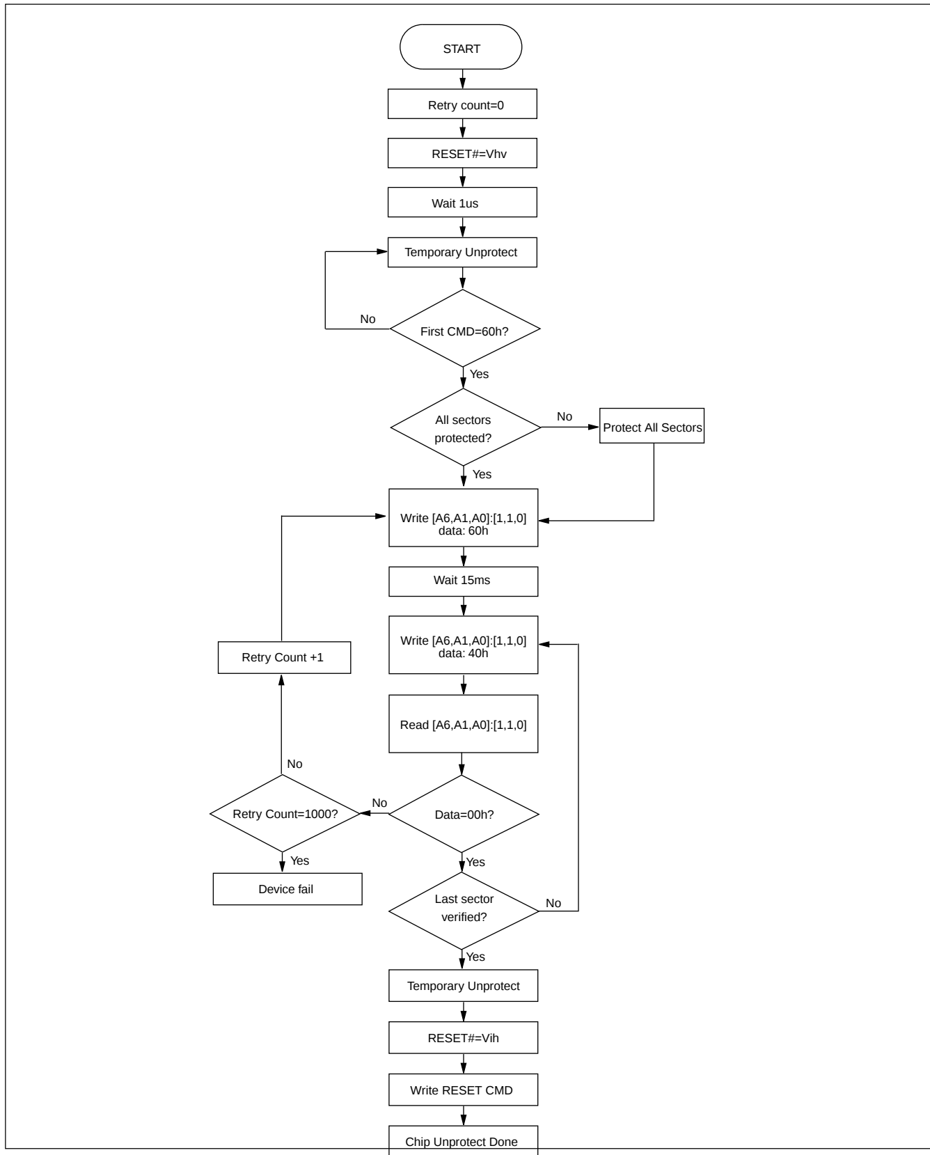
Figure 15. CHIP UNPROTECT ALGORITHMS WITH RESET# = V h v
