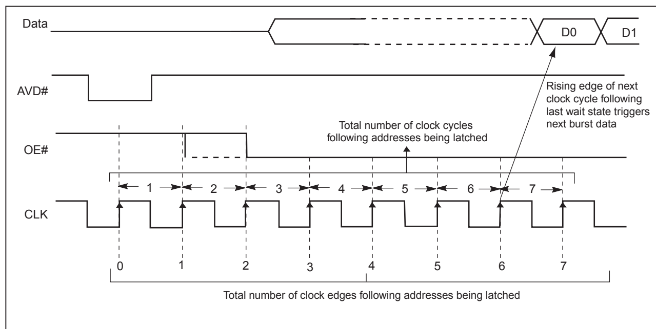
Figure 4. Example of Programmable Dummy Cycles
