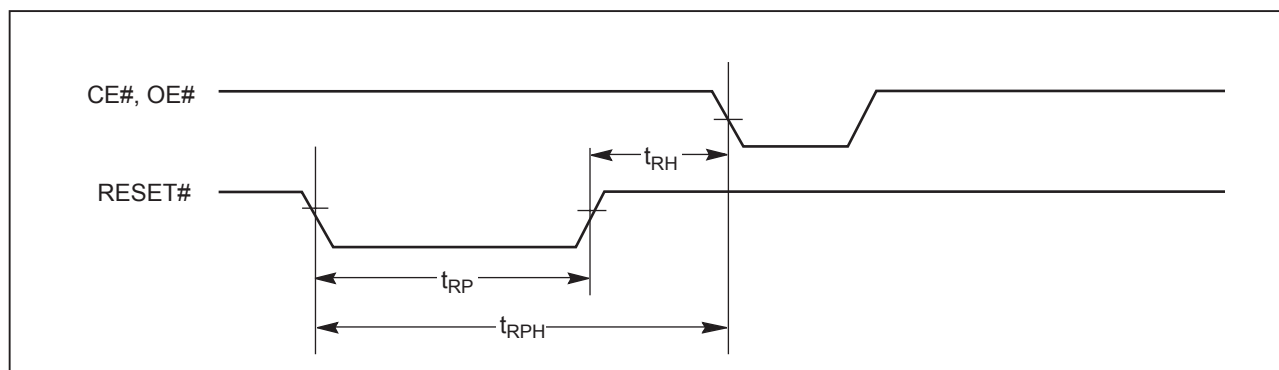
Figure 5. Reset Timings
