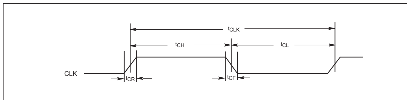
Figure 10. CLK Characterization
