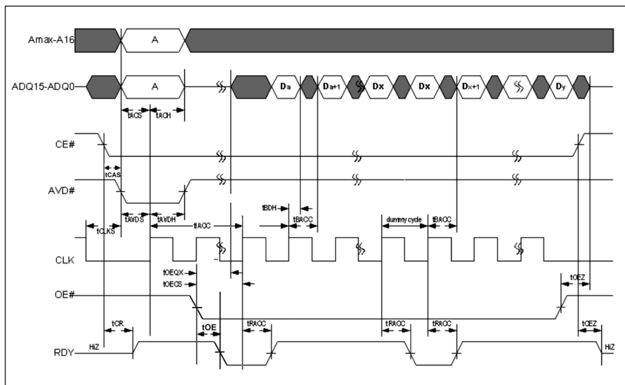
Figure 11. Burst Mode Read
