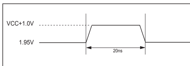
Maximum Negative Overshoot Waveform
