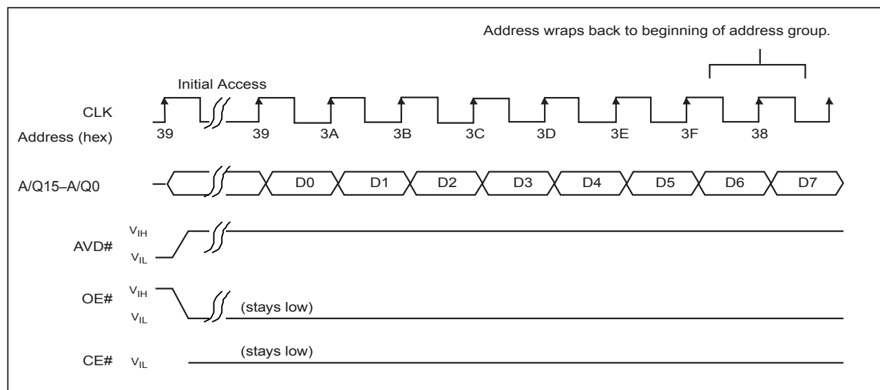
Figure 15. 8-, 16-Word Linear Burst Address Wrap Around
