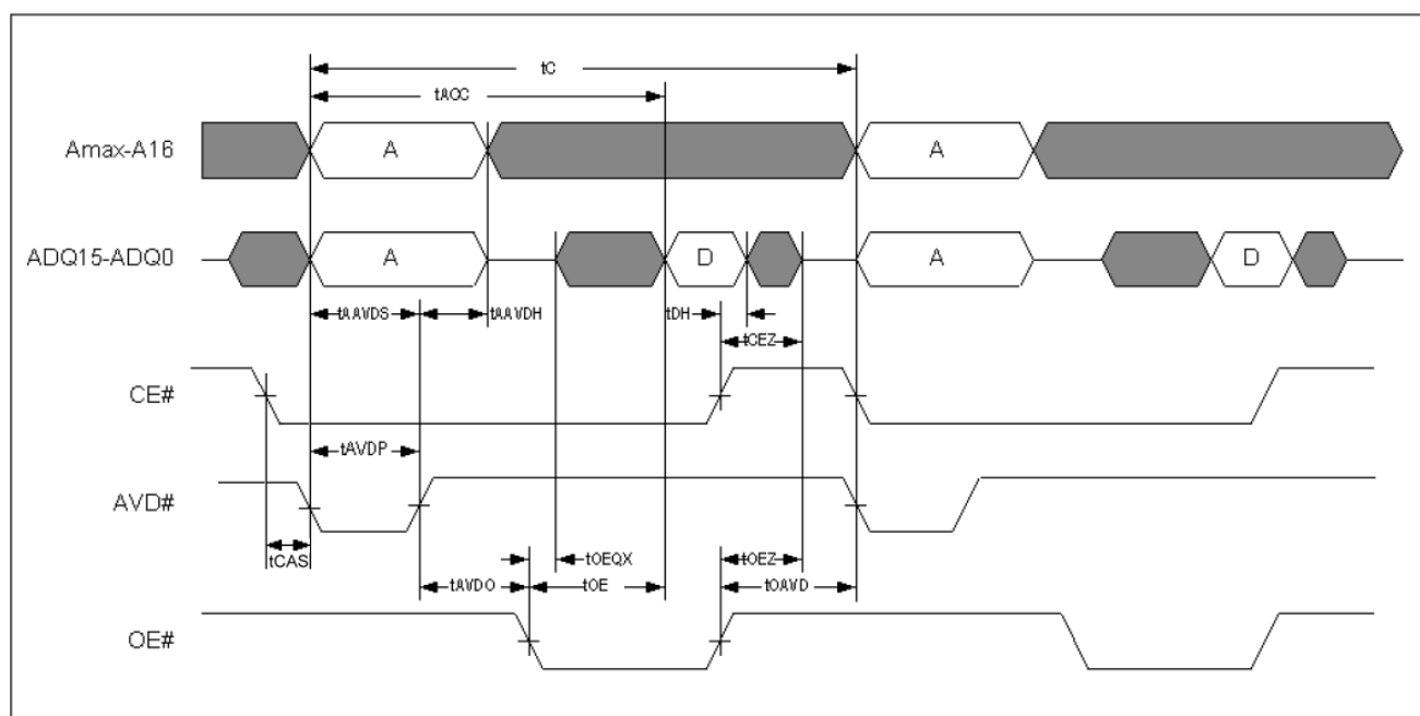
Figure 12. Asynchronous Mode Read
