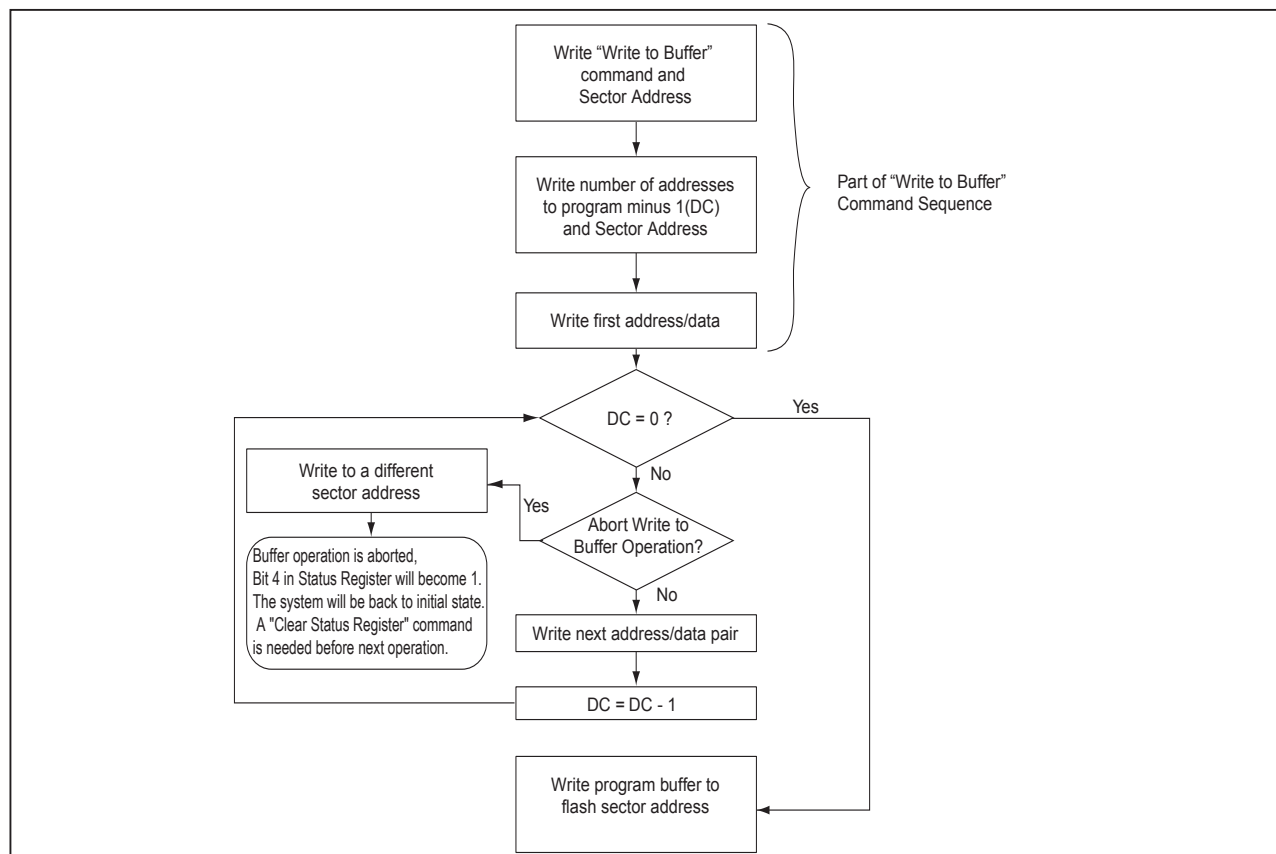
Figure 2. Write Buffer Programming Operation
