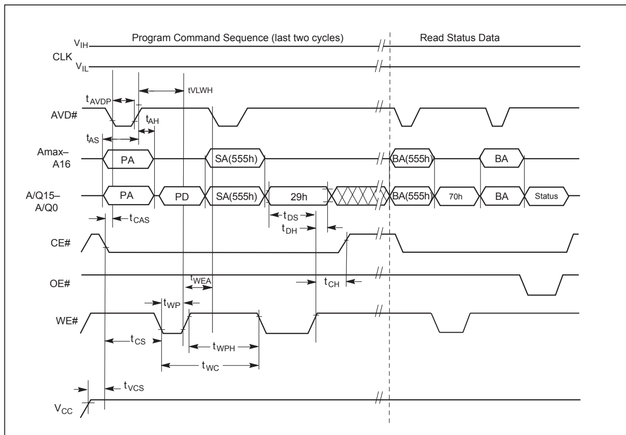
Figure 13. Program Operation Timings
