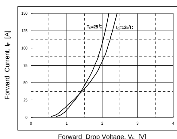
Fig 12. Forward characteristics
