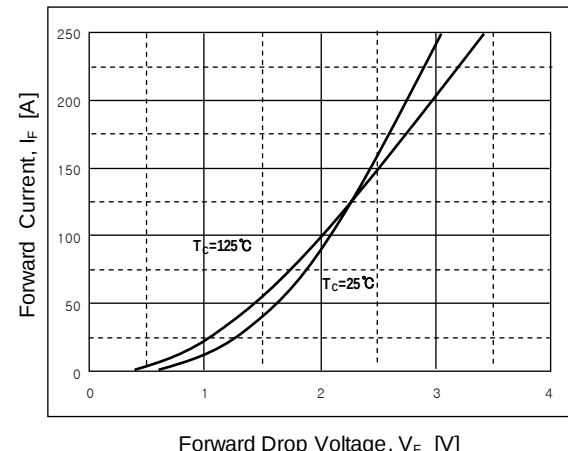
Fig 12. Forward characteristics
