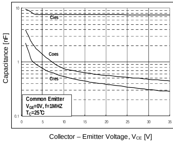
Fig 7. Capacitance characteristics
