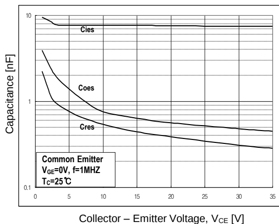
Fig 7. Capacitance characteristics
