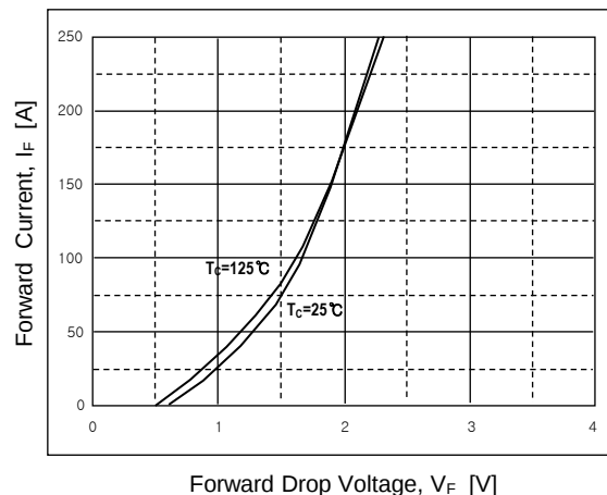
Fig 12. Forward characteristics
