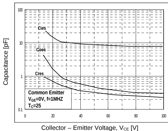
Fig 7. Capacitance characteristics
