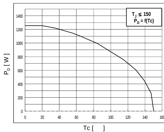
Fig 10. Power Dissipation vs. Case Temperature
