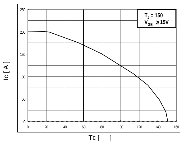
Fig 9. rated Current vs. Case Temperature
