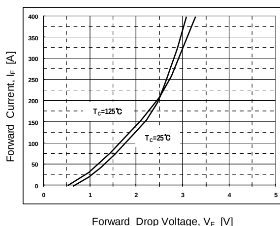
Fig 12. Forward characteristics
