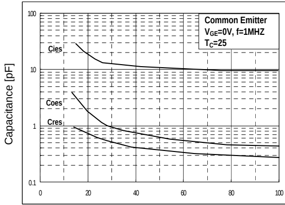
Collector - Emitter Voltage, V_{CE} [V] Fig 7. Capacitance characteristics
