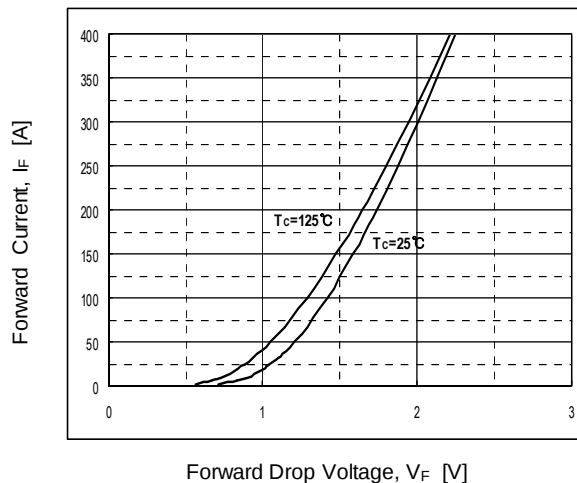
Fig 14. Forward characteristics
