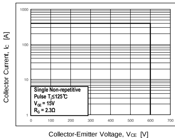
Fig 9. RBSOA Characteristic
