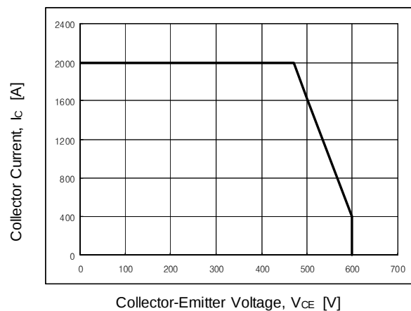
Fig 10. SCSOA Characteristic
