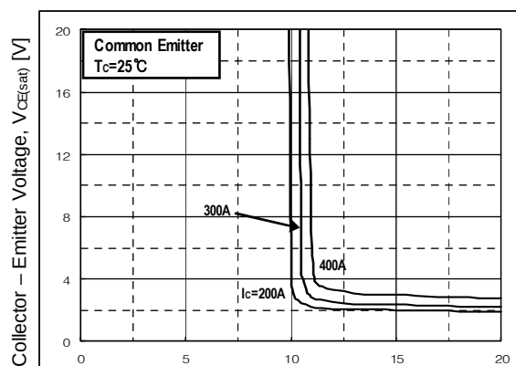
Fig 3. Typical Saturation Voltage characteristics
