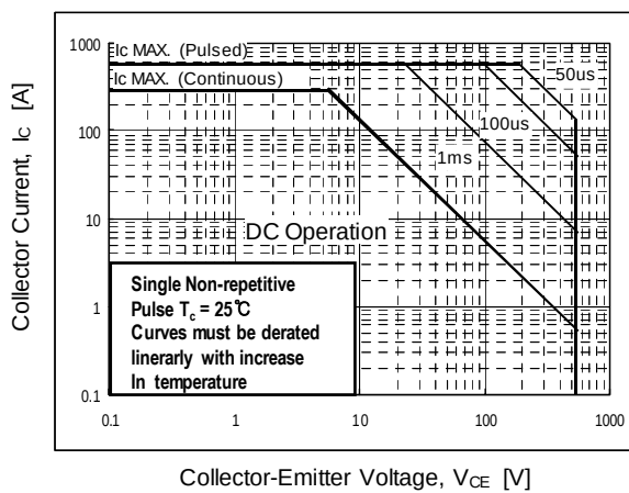
Fig 11. SOA Characteristic
