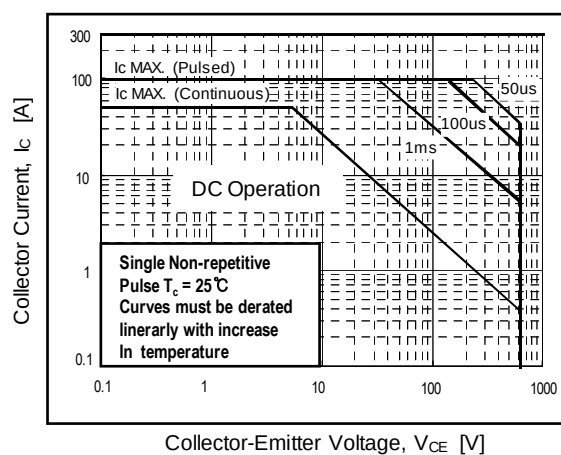
Fig14. SOA characteristics
