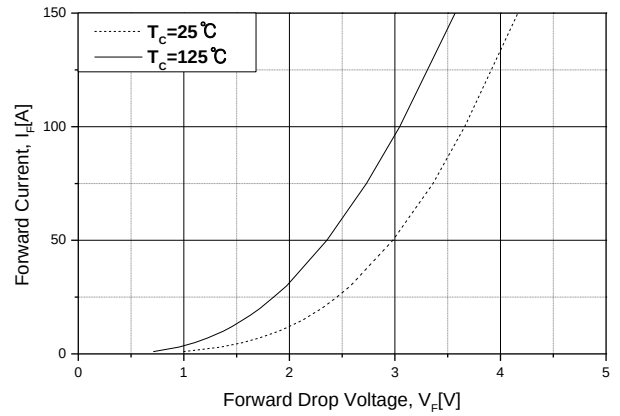
Fig.10 Forward Characteristics
