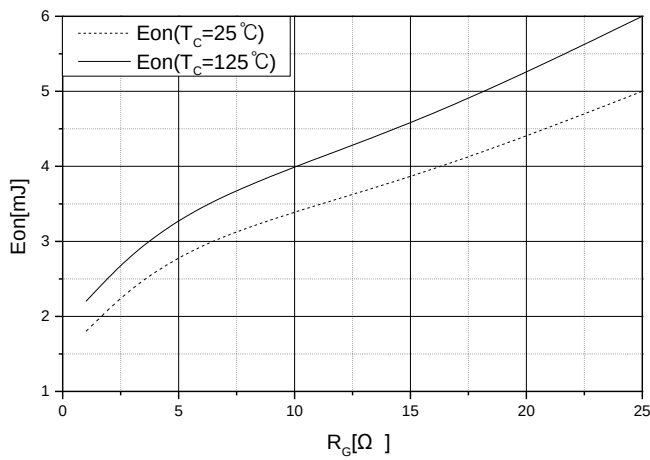
Fig.5 Typical turn-on energy = f(R_G) V_{GE} = \pm 15V, I_C = 50A, V_{CE} = 600V
