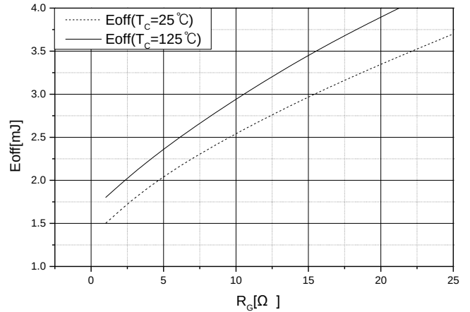
Fig.6 Typical turn-off energy = f(R_G) V_{GE} = \pm 15V, I_C = 50A, V_{CE} = 600V
