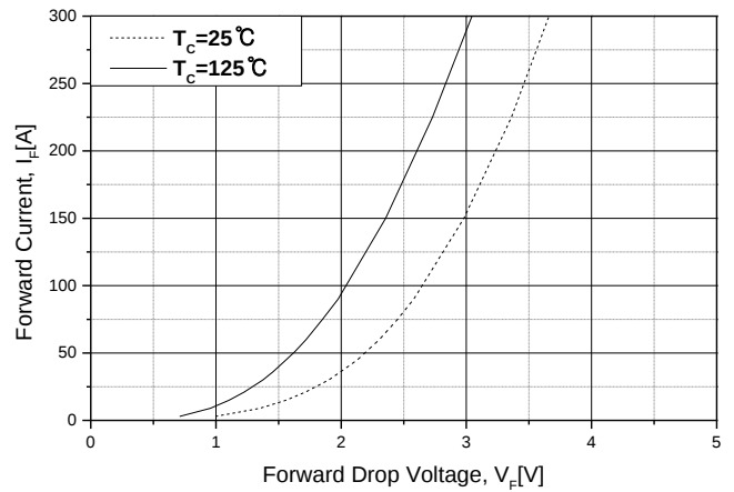
Fig.10 Forward Characteristics
