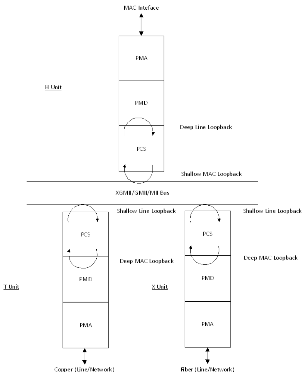
Figure 5: Loopback Paths
