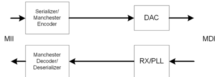
Figure 17: 10BASE-T Data Path
