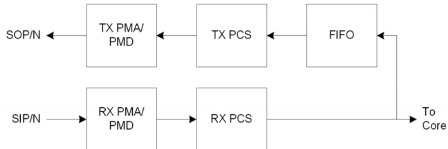
Figure 20: Shallow Host Loopback
