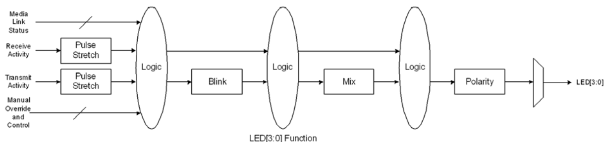
Figure 10: LED Chain
