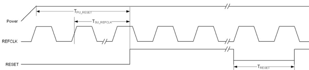
Figure 23: Reset Timing
