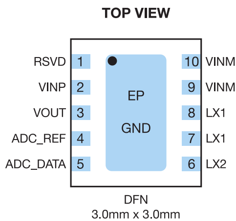
Figure 3: Package diagram for 10-lead, 3mm x 3mm DFN
