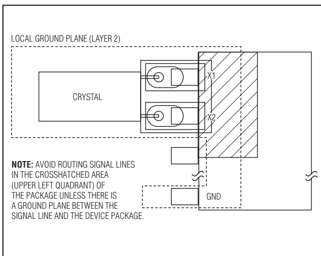
Figure 8. Layout Example
