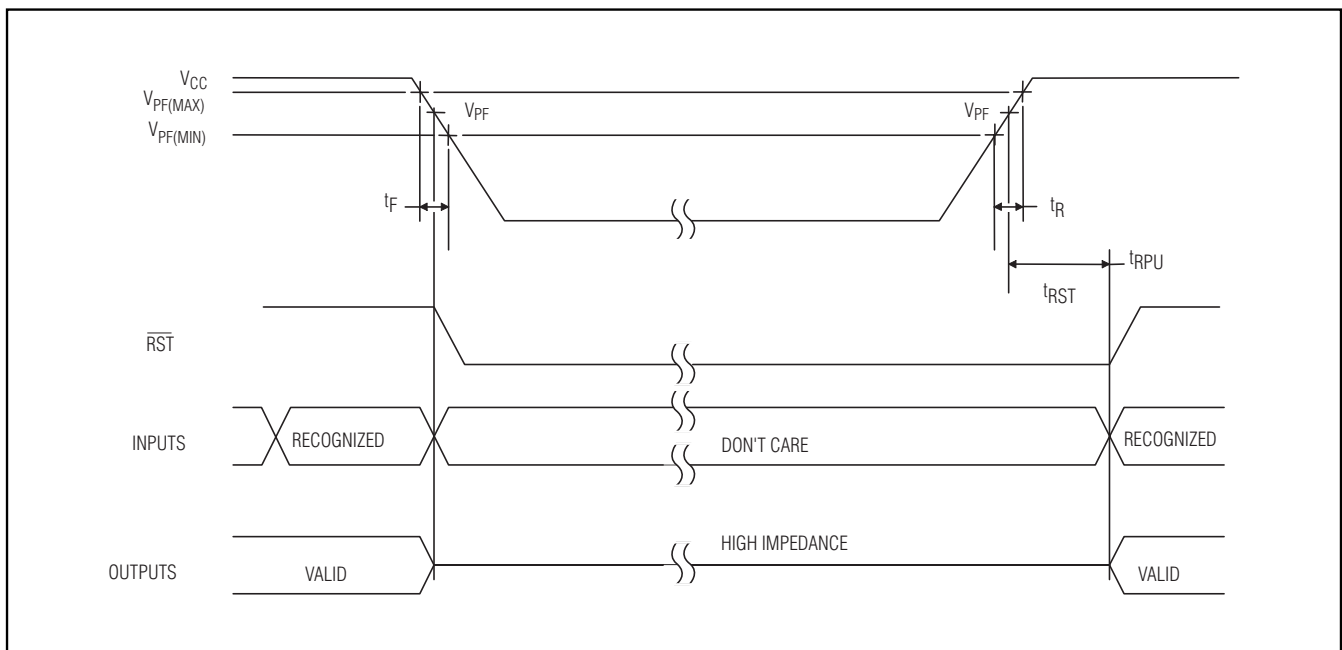
Figure 5. Power-Up/Down Timing
