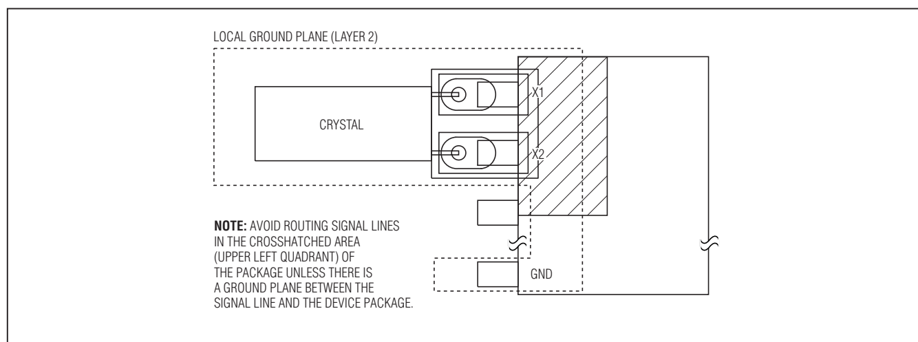
Figure 7. Layout Example
