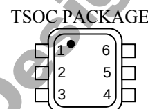
TOP VIEW 3.7mm x 4.0mm x 1.5mm
