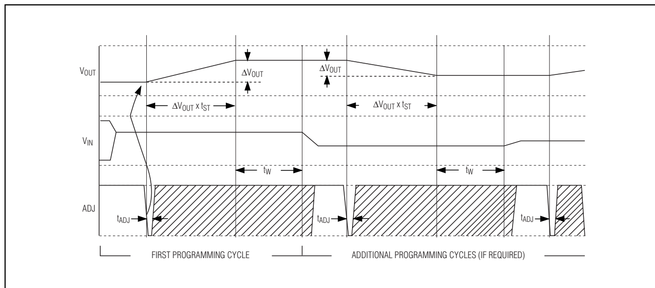
Figure 1. Timing Diagram
