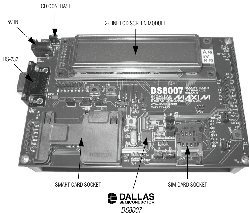
Figure 1. DS8007 Evaluation Kit
