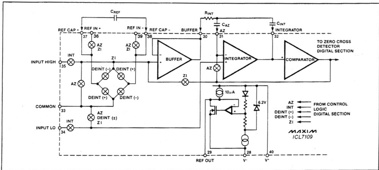
Figure 2. Analog Section
