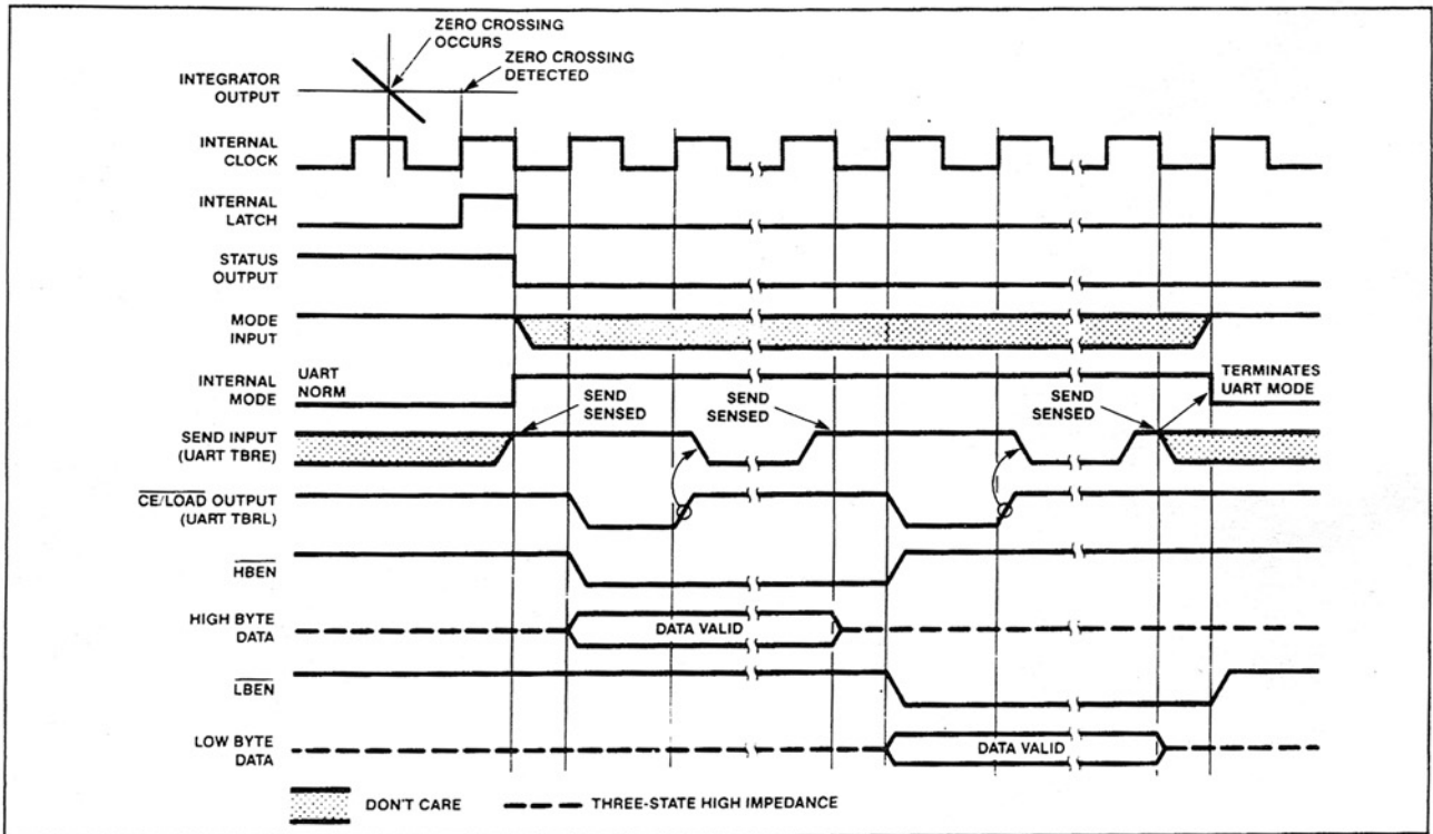
Figure 10. Handshake - Typical UART Interface Timing
