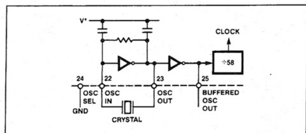
Figure 7. Crystal Oscillator
