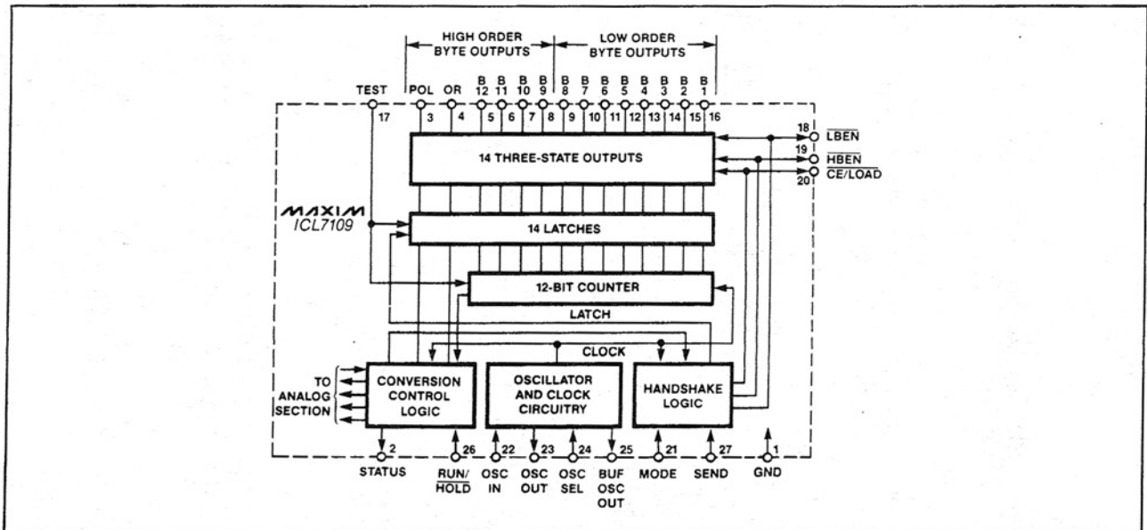
Figure 4. Digital Section
