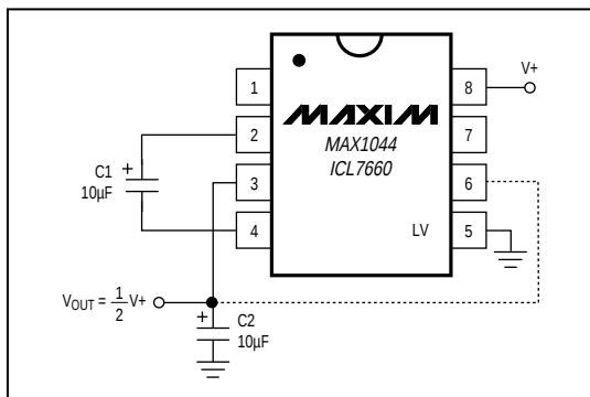
Figure 10. Voltage Divider
