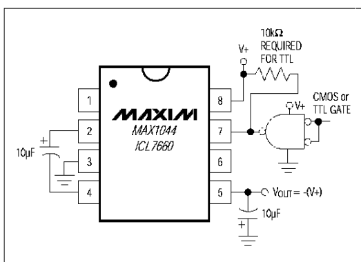
Figure 7. External Clocking
