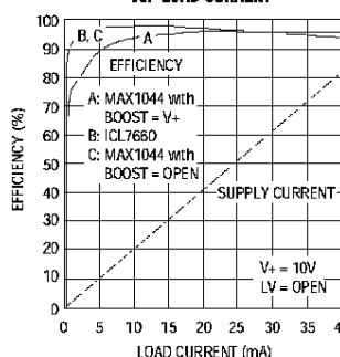
EFFICIENCY and SUPPLY CURRENT vs. LOAD CURRENT
