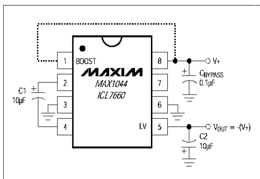
Figure 8. Negative Voltage Converter with BOOST and LV Connections
