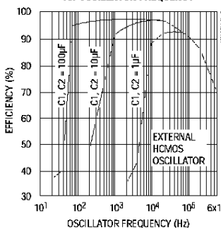
EFFICIENCY vs. OSCILLATOR FREQUENCY
