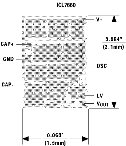
TRANSISTOR COUNT: 71 SUBSTRATE CONNECTED TO V+
