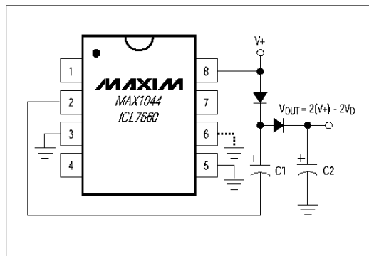
Figure 9. Voltage Doubler
