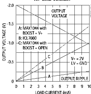
OUTPUT VOLTAGE and OUTPUT RIPPLE vs. LOAD CURRENT
