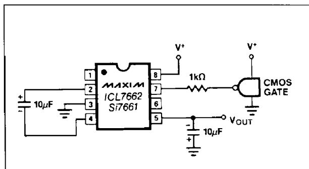
Figure 4. External Clocking
