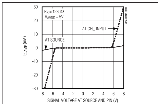
Figure 3. Input Clamp Characteristics (Zoom In)
