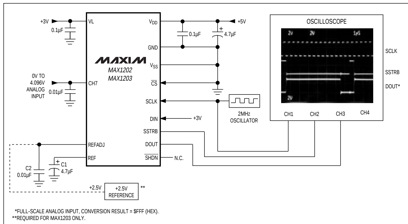
Figure 5. Quick-Look Circuit
