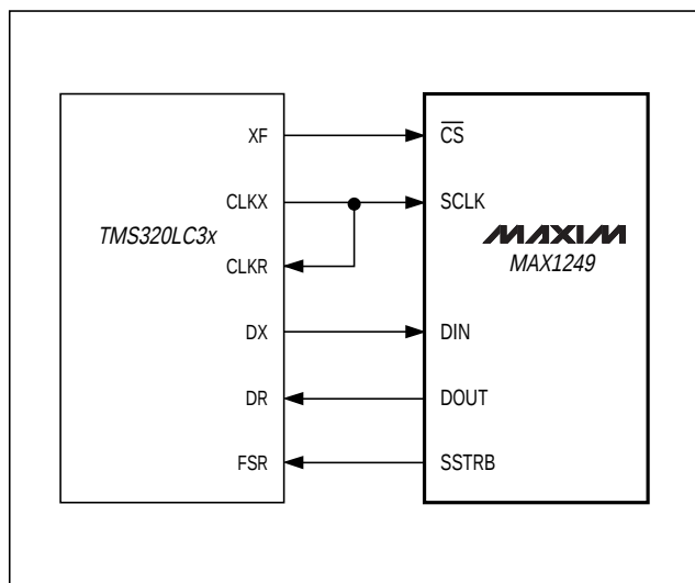
Figure 20. MAX1248/MAX1249-to-TMS320 Serial Interface
