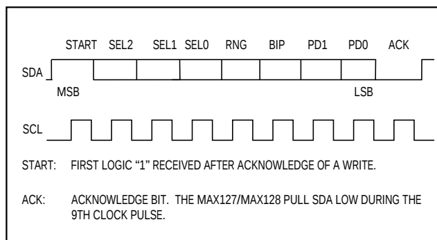
Figure 8. Command Byte
