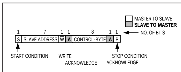
Figure 6. Write Cycle
