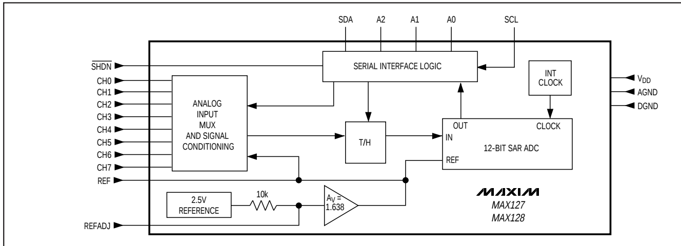
Figure 1. Block Diagram
