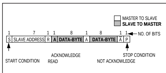
Figure 7. Read Cycle
