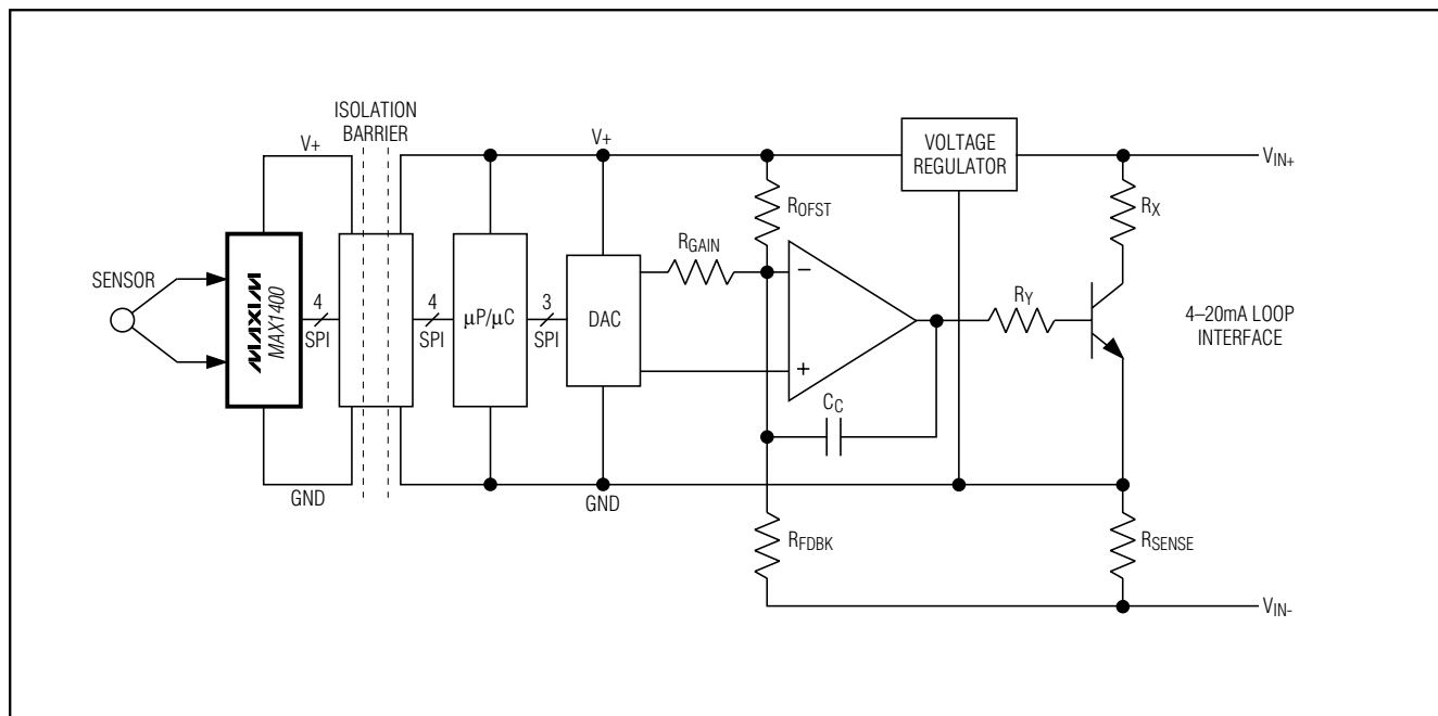
Figure 18. 4–20mA Transmitter
