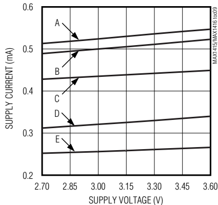
SUPPLY CURRENT vs. SUPPLY VOLTAGE (MAX1415)
