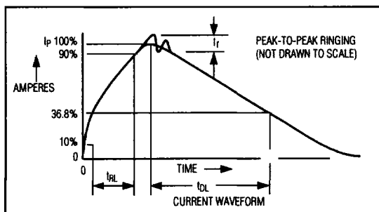
Figure 2b. Human Body Model Current Waveform
