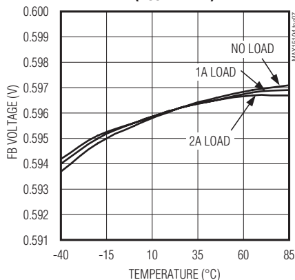
FB VOLTAGE vs. TEMPERATURE ( V_{OUT} = 1.5V )
