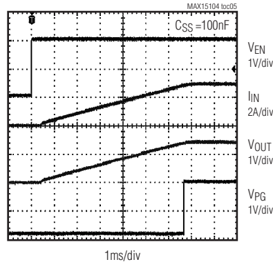
STARTUP WAVEFORMS
