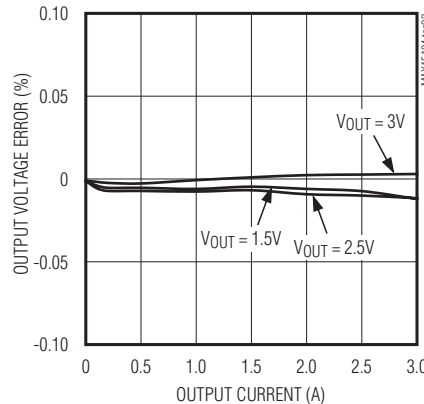
OUTPUT VOLTAGE ERROR vs. OUTPUT CURRENT
