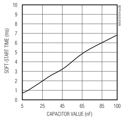
SOFT-START TIME vs. CAPACITOR VALUE
