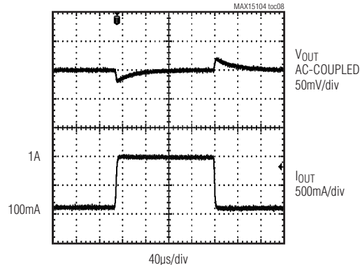
1A LOAD-TRANSIENT RESPONSE
