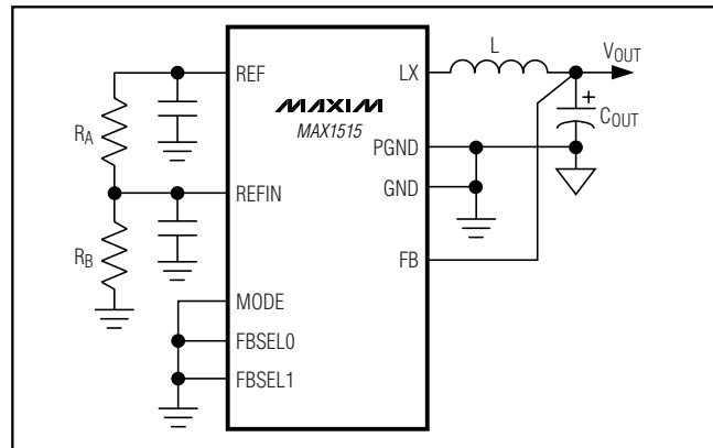
Figure 5. Setting V_{OUT} with a Resistive Voltage-Divider at REF
