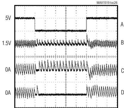
SINGLE-PHASE SKIP TO DUAL-PHASE PWM TRANSITION
