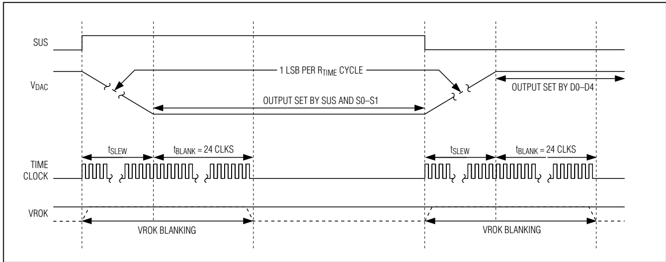
Figure 4. Suspend Transition
