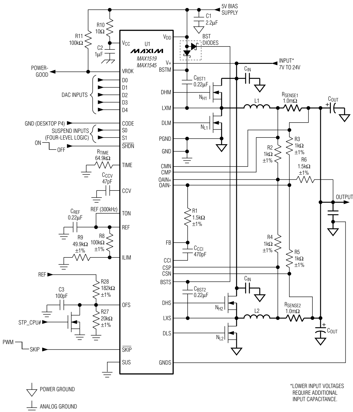
Figure 1. Standard Two-Phase Desktop P4 Application Circuit
