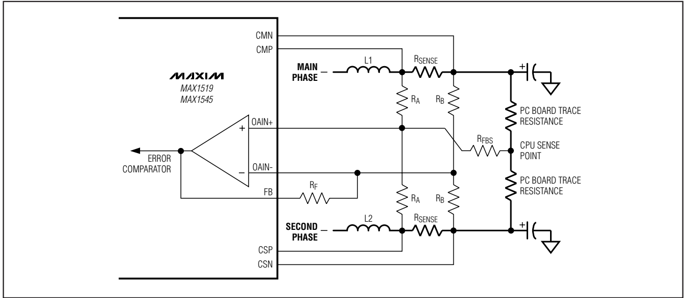
Figure 10. Voltage-Positioning Gain
