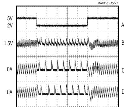
DUAL-PHASE SKIP TO DUAL-PHASE PWM TRANSITION
