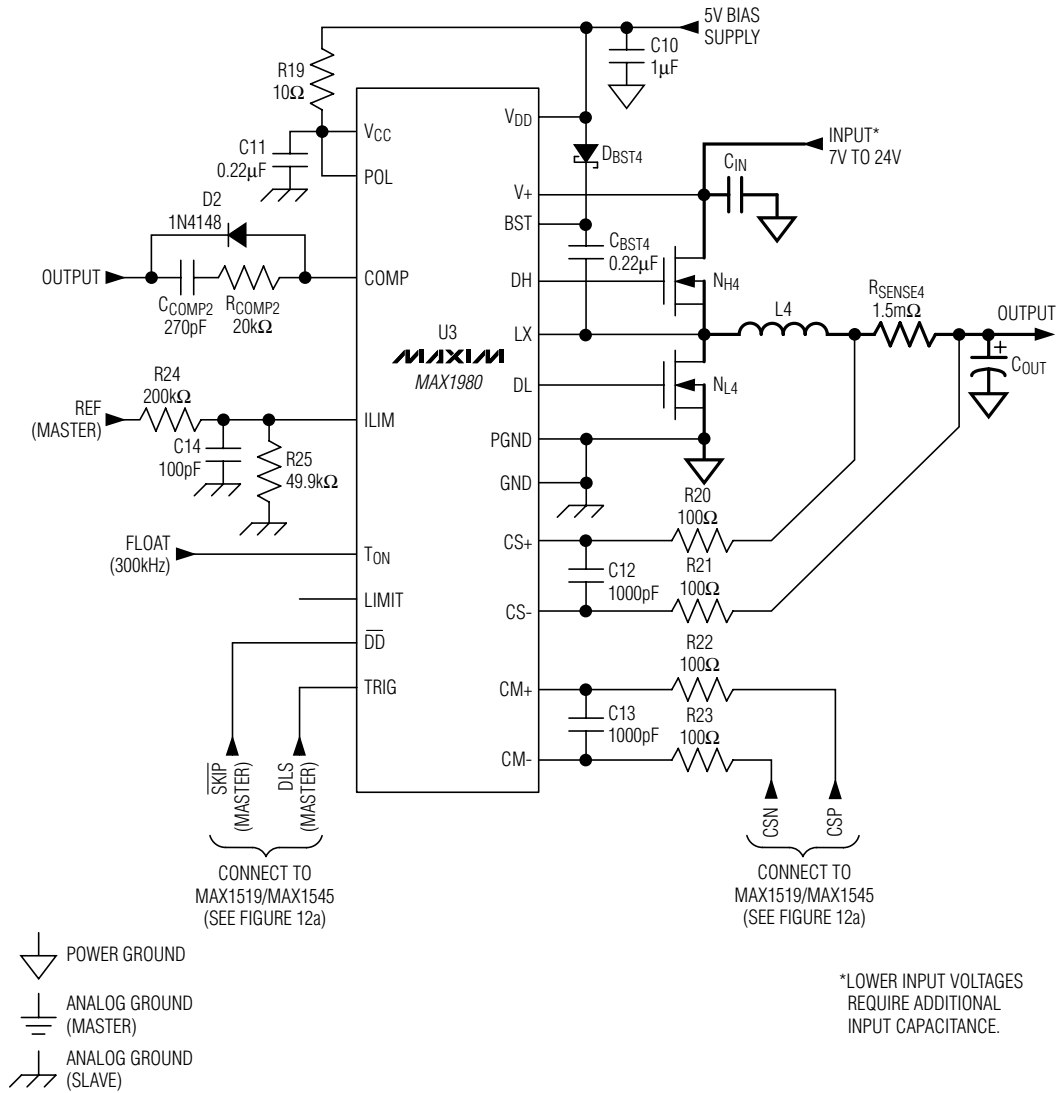
Figure 12c. Standard 4-Phase Desktop 4 Application Circuit (4th Phase—MAX1980 Slave)
