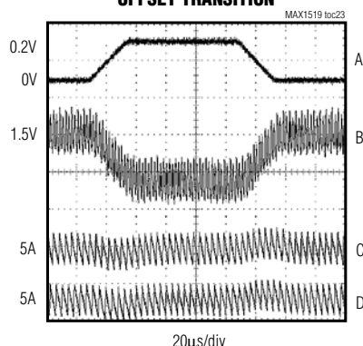
OFFSET TRANSITION
