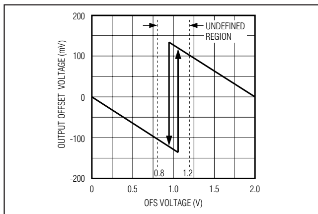
Figure 6. Offset Voltage
