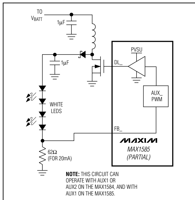
Figure 6. AUX_ Channel Powering a White LED Step-Up Current Source
