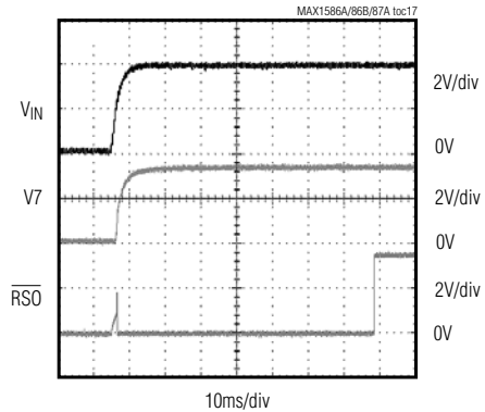
V7 AND R50 STARTUP WAVEFORMS
