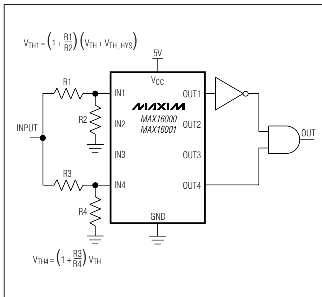
Figure 8. Window Detection
