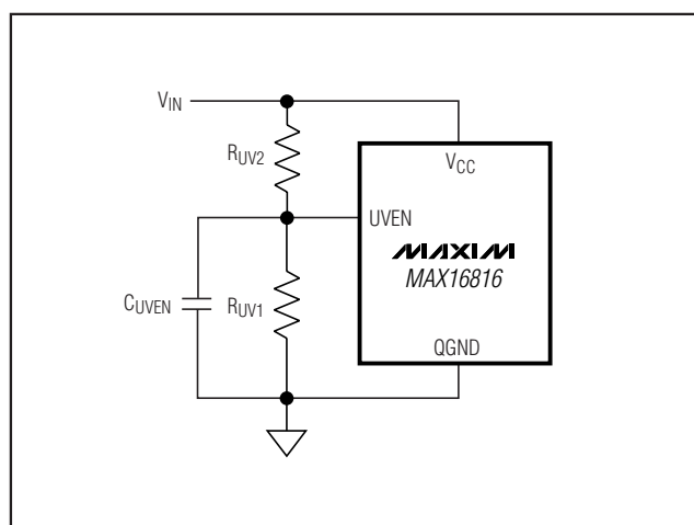
Figure 1. Setting the UVLO Threshold
