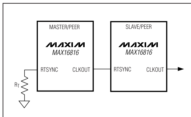
Figure 3. Master-Slave/Peer-Peer Clock Configuration
