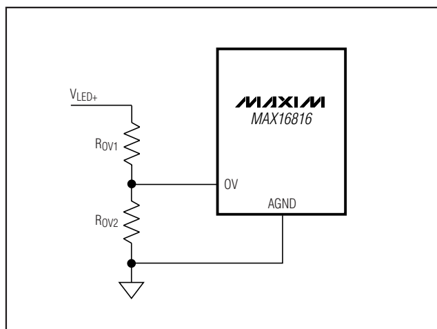
Figure 4. Setting the Overvoltage Threshold
