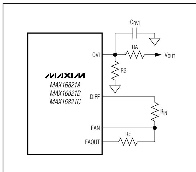
Figure 4. Overvoltage Protection Input Delay
