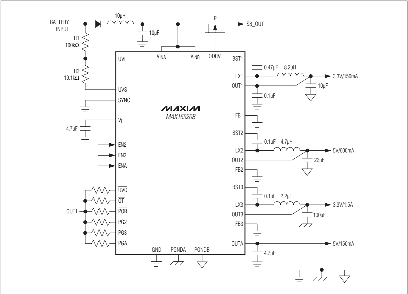
Figure 5. Typical Operating Circuit for MAX16920BATJ/V+ Operating at 2.2MHz
