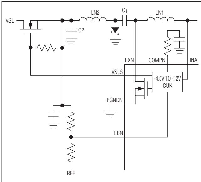
Figure 3. Cuk Converter
