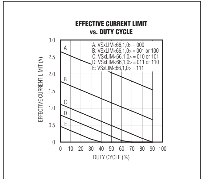
Figure 4. Effective Current Limit vs. Duty Cycle
