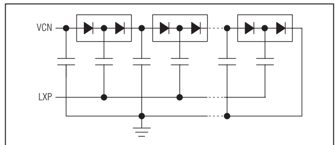
Figure 8. Multistage Inverting Charge Pump for Negative Output (Cuk is Inactive)
