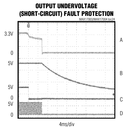
A. 3.3V OUTPUT ( V_{OUT3} ), 2V/div B. 5V OUTPUT ( V_{OUT5} ), 2V/div C. PGDALL, 5V/div D. DL3, 5V/div
